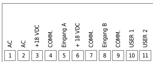
Connections PAXDP
